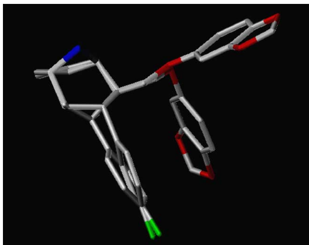
Figure 5. A superimposition of the X-ray crystal structures of 4a and 4d .
