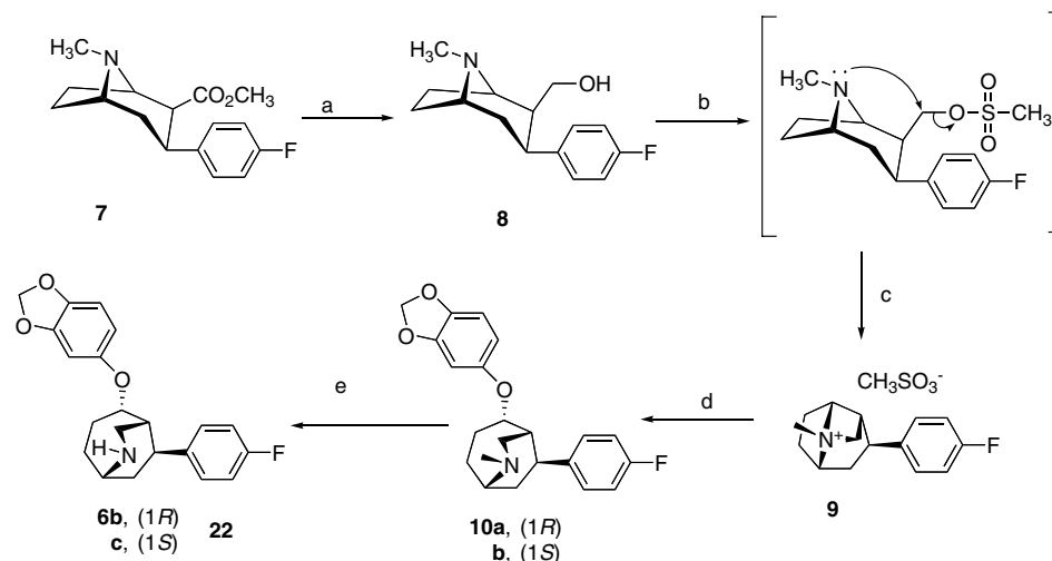
Scheme 1. Reagents and conditions: (a) \text{LiAlH}_4 , THF, 0^\circ\text{C} ; (b) (1) methanesulfonyl chloride, TEA, 0^\circ\text{C} ; (c) toluene, 1 h reflux; (d) Na, sesamol, THF, reflux; (e) (1) 1-chloroethyl chloroformate, 1,2-dichloroethane, 24 h reflux; (2) MeOH, 24 h reflux.
