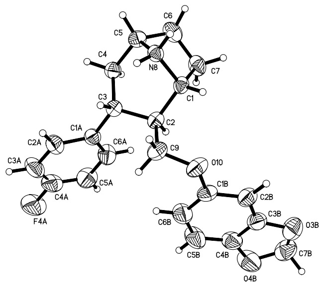
Figure 3. Structure of compound 4d as determined by X-ray diffraction. Thermal ellipsoids are shown at the 30% probability level, hydrogen atoms are shown as circles of an arbitrary radius.
