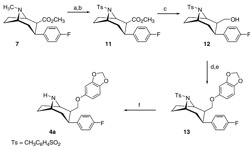
Scheme 2. Reagents and conditions: (a) (1) 1-chloroethyl chloroformate, 1,2-dichloroethane, reflux; (2) MeOH reflux; (b) p -toluenesulfonyl chloride, triethylamine; (c) \text{LiAlH}_4 , THF, rt; (d) trifluoromethanesulfonic anhydride, pyridine, \text{CH}_2\text{Cl}_2 ; (e) Na, sesamol, THF; (f) 5% Na/Hg amalgam, \text{Na}_2\text{HPO}_4 , MeOH.
