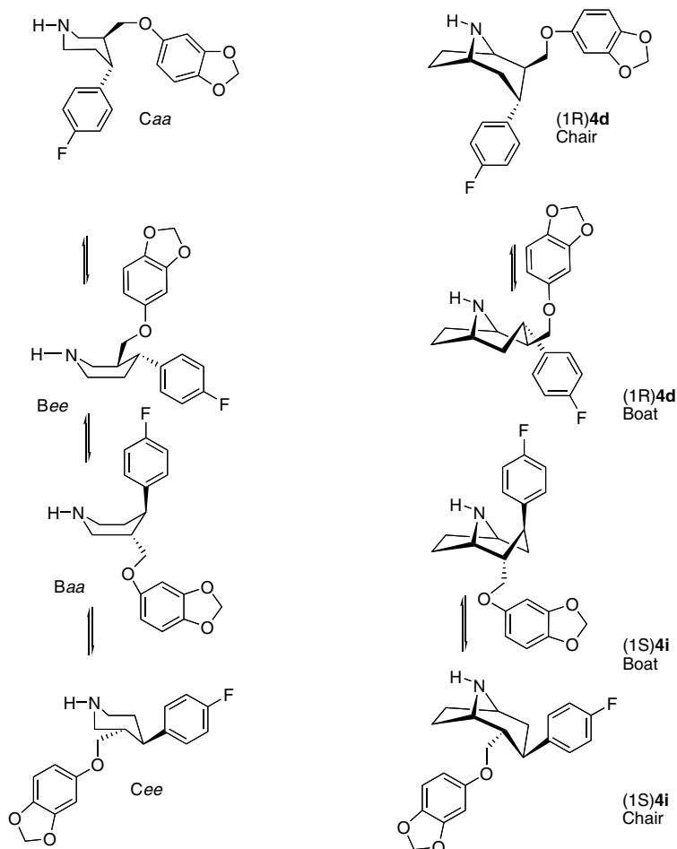
Figure 4. Potential conformations of paroxetine 2 and the analogous tropanes 4d and 4i . B and C indicate boat and chair conformations while aa and ee are axial–axial and equatorial–equatorial.
