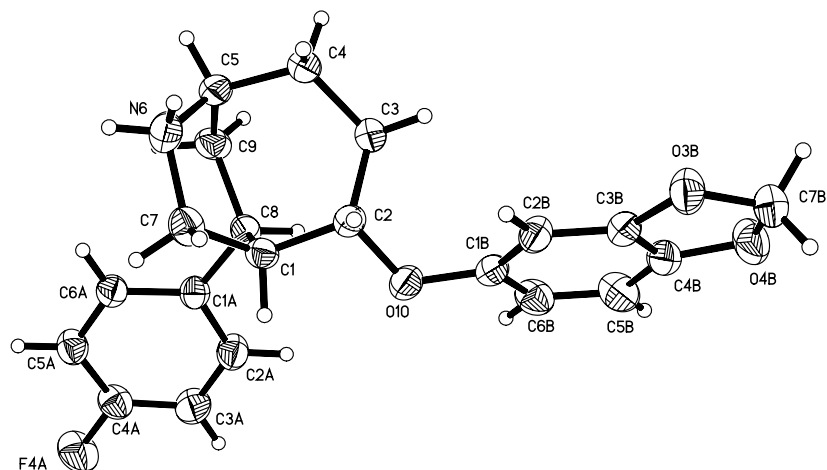
Figure 1. Structure of compound 6b as determined by X-ray diffraction. Thermal ellipsoids are shown at the 30% probability level, hydrogen atoms are shown as circles of an arbitrary radius.
